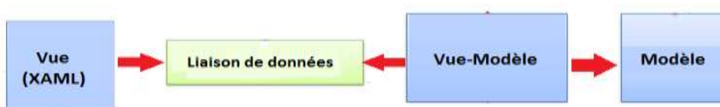
Figure 81. Model View-View Model
