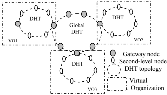
Figure 2: A single gateway hierarchical DHT Architecture (SG-HDHT).
