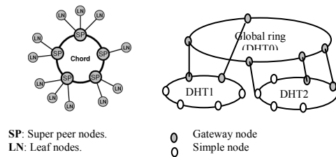
Figure 1: SP-HDHT (left) and MG-HDHT (right) solutions.
