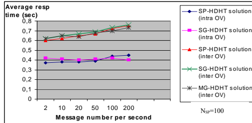
Figure 5: Comparison between SP-HDHT, MG-HDHT and SG-HDHT performances.
