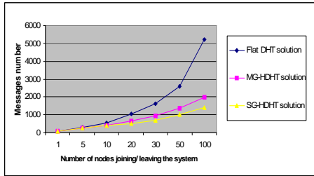
Figure 6: Impact of the connection / disconnection of nodes in the messages number exchanged in the system.
