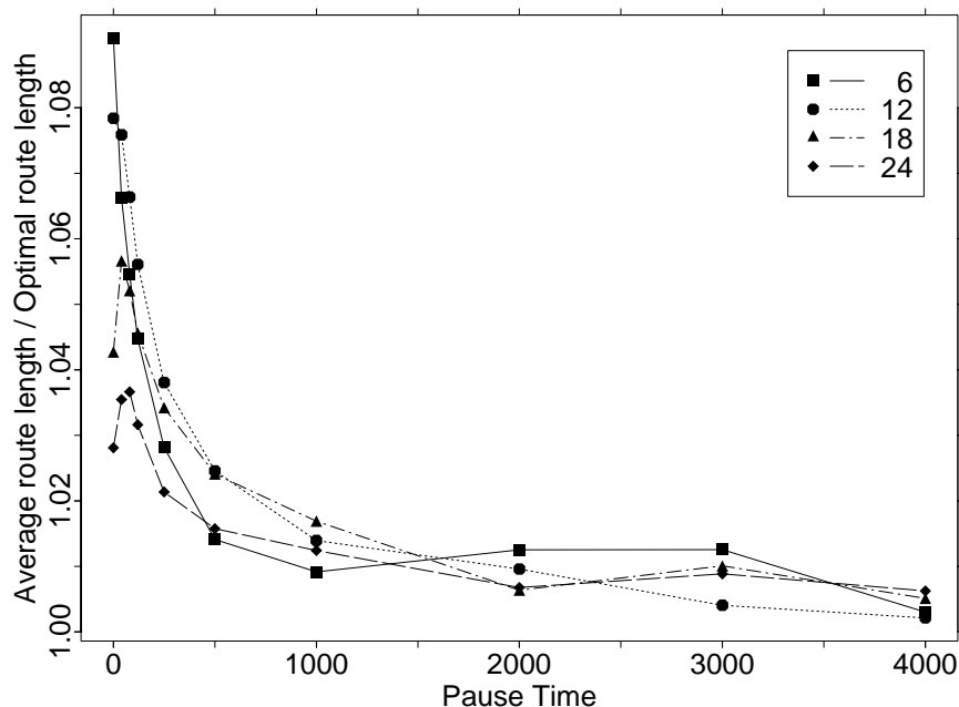
Figure 8 Average route length used relative to optimal
