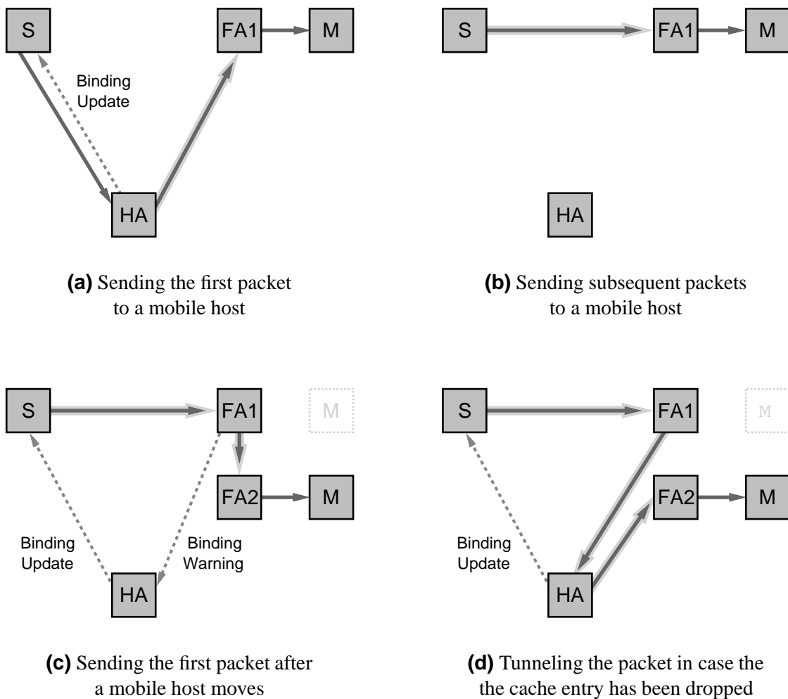
Figure 4 Operation of the Route Optimization protocol extensions
