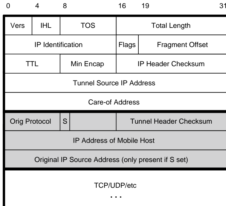
Figure 3 Mobile IP tunneling using “minimal” encapsulation
