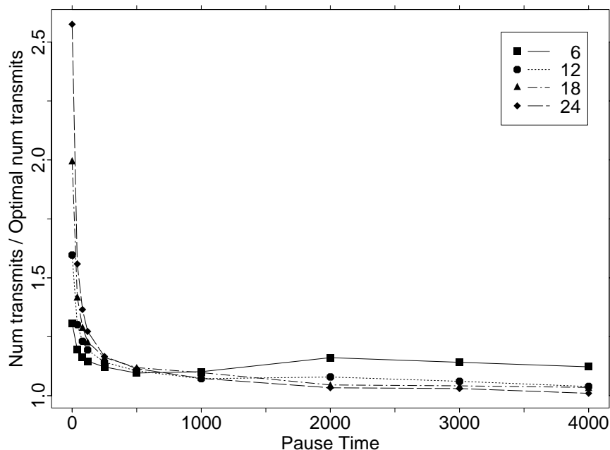
Figure 7 Average total number of transmissions performed relative to optimal
