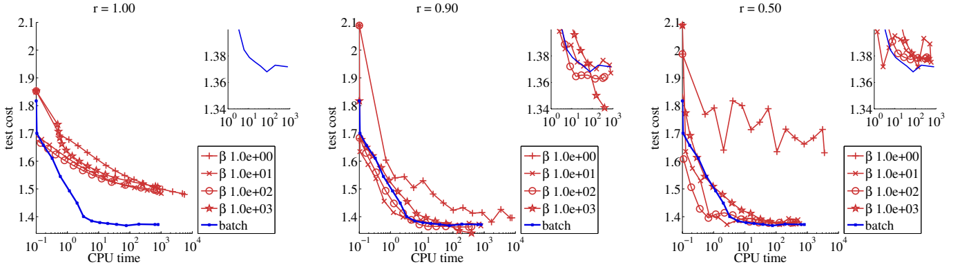
Figure 1: Comparison of online and batch algorithm on a thirty-seconds long audio track.
