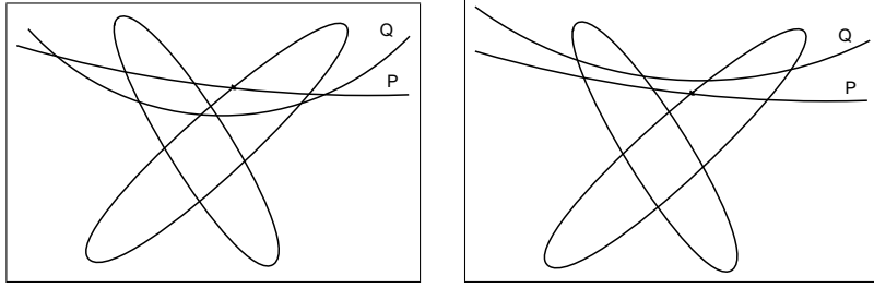
Figure 1: Broccoli semantics of the counterfactual operators [\varphi]\psi and [\varphi]\rangle\psi , with |\varphi| = P and |\psi| = Q .
