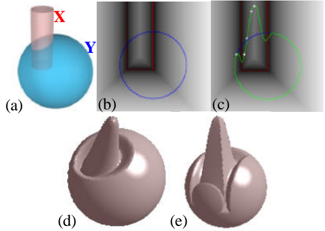
Figure 13: (a) The sphere (ordinate and direction) is sculpted around a cylindrical (abscissa and support) tool, (b) representation in our 2D interface ,(c) a profile is defined by the user, (d) the extrusion support is now a parallelepiped.
