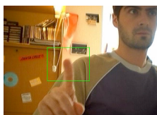
Figure 4: Index tracking
