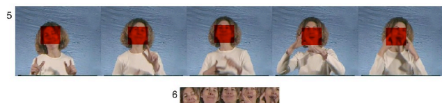
Figure 5: Face tracking
