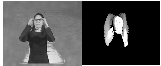
Figure 6: Arm movements
