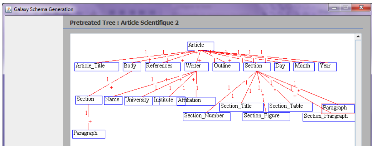
Figure 6: Pretreated tree with added cardinalities.
