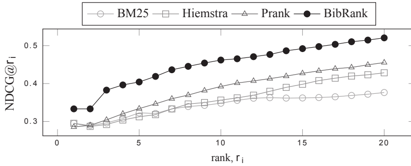
Fig. 12: NDCG at different author ranking
