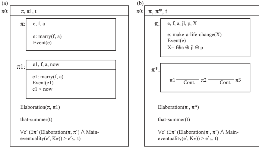
Figure 8. SDRS for example (10) (a) First step in building the SDRS (b) Resulting SDRS
