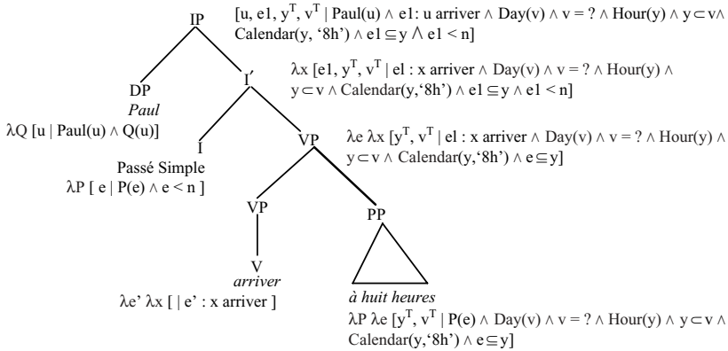
Figure 3. Compositional semantics of (6)
