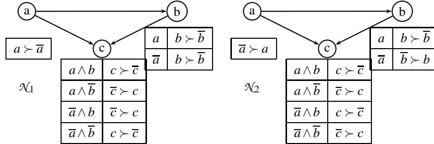
Figure 1: CP-net of Players 1 and 2's preferences for G^*
