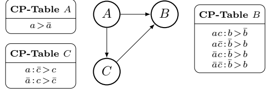
Figure 1: A deterministic CP-net
