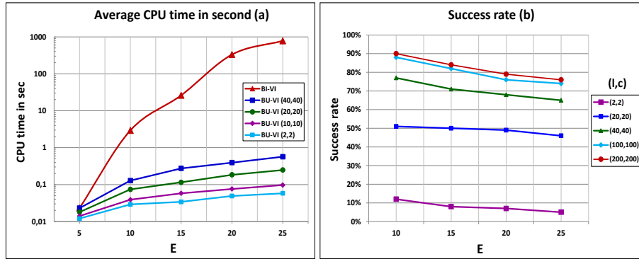
Figure 2: Bounded utility lexicographic value iteration VS lexicographic value iteration
