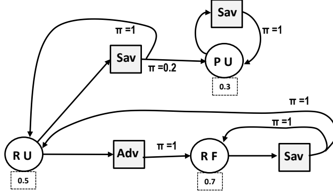
Figure 1: The stationary IIMDP of Example 2
