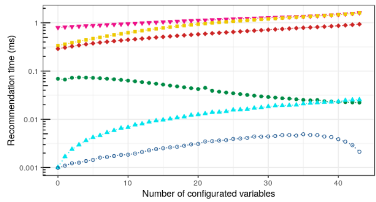
Legend ● Classical Bayes ▼ Weighted Majority Voter ◆ Naive Bayes Voter ▲ Naive Bayes ■ Most Popular Choice ○ 3-LP-tree (3 cl.)
