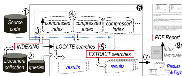
Figure 1: Workflow in uiHRDC to reproduce experiments.
