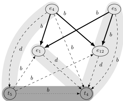
Figure 1: The full temporal graph for the Aquaint excerpt. Labels b and d stand for before and during .
