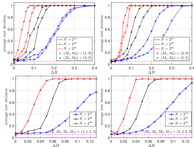
Fig. 4: Power of the test. Empirical assessment of the test powers, obtained as average of the decision of the bootstrap test, as a function of \Delta H , for M = 4 (left) and M = 10 (right), for different sample sizes, and with equal or different sizes in the groups of equal components, for Scenario1 (top) and Scenario2 (bottom). Significance level is set to \alpha = 0.05 (magenta dashed line).
