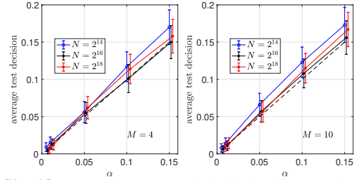
Fig. 3: Significance levels. Empirical significance levels (obtained as averages of the bootstrap test decisions against targeted ones) against targeted ones.
