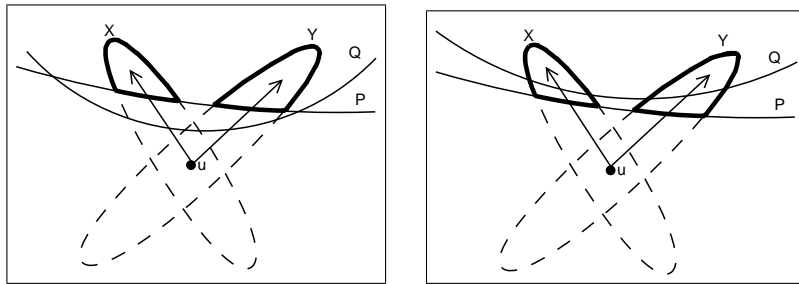
Figure 4: Intended semantics of the Broccoli revision operators [\varphi]\psi and [\varphi]\psi , with |\varphi| = P and |\psi| = Q .
