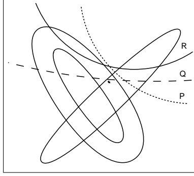
Figure 5: Counter-model to \langle \varphi \rangle \psi \rightarrow ([\varphi](\psi \rightarrow \theta) \rightarrow [\varphi \wedge \psi]\theta) , with P = |\theta| , Q = |\varphi| and R = |\psi| .
