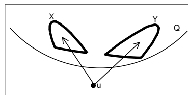
Figure 2: Minimal relational model
