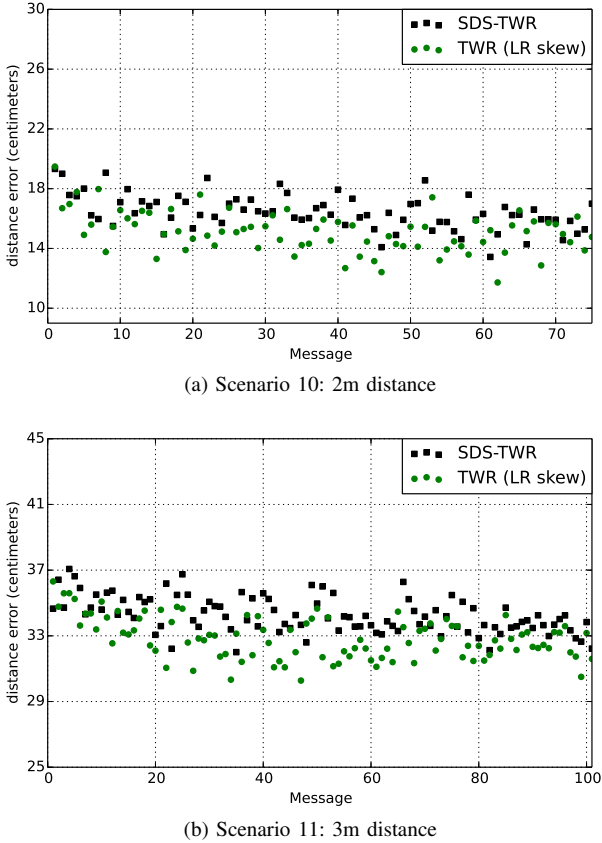
Fig. 10: SDS-TWR vs TWR with skew comparison
