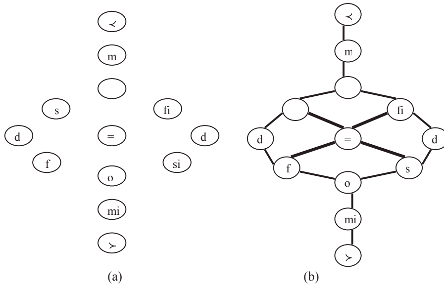
Figure 1: Allen's thirteen primitive relations arranged according to their conceptual neighborhood.
