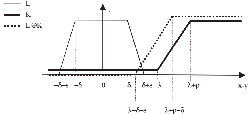
Figure 3: Modeling "approximate equality" and "graded strict inequality".
