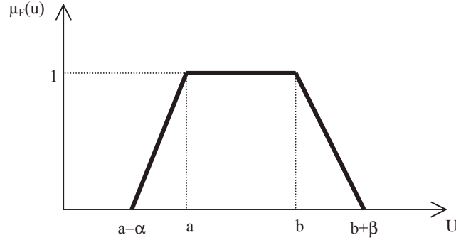
Figure 2: Trapezoidal membership function
