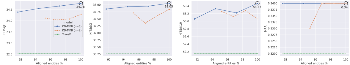
Figure 4: HITS@1, HITS@3, HITS@10 and MRR link prediction results for KD-MKB using FB15K-237 when different sizes of the alignment set ( I_e(i, j) ) are used. Our best performances are highlighted by a circle and values were included.
